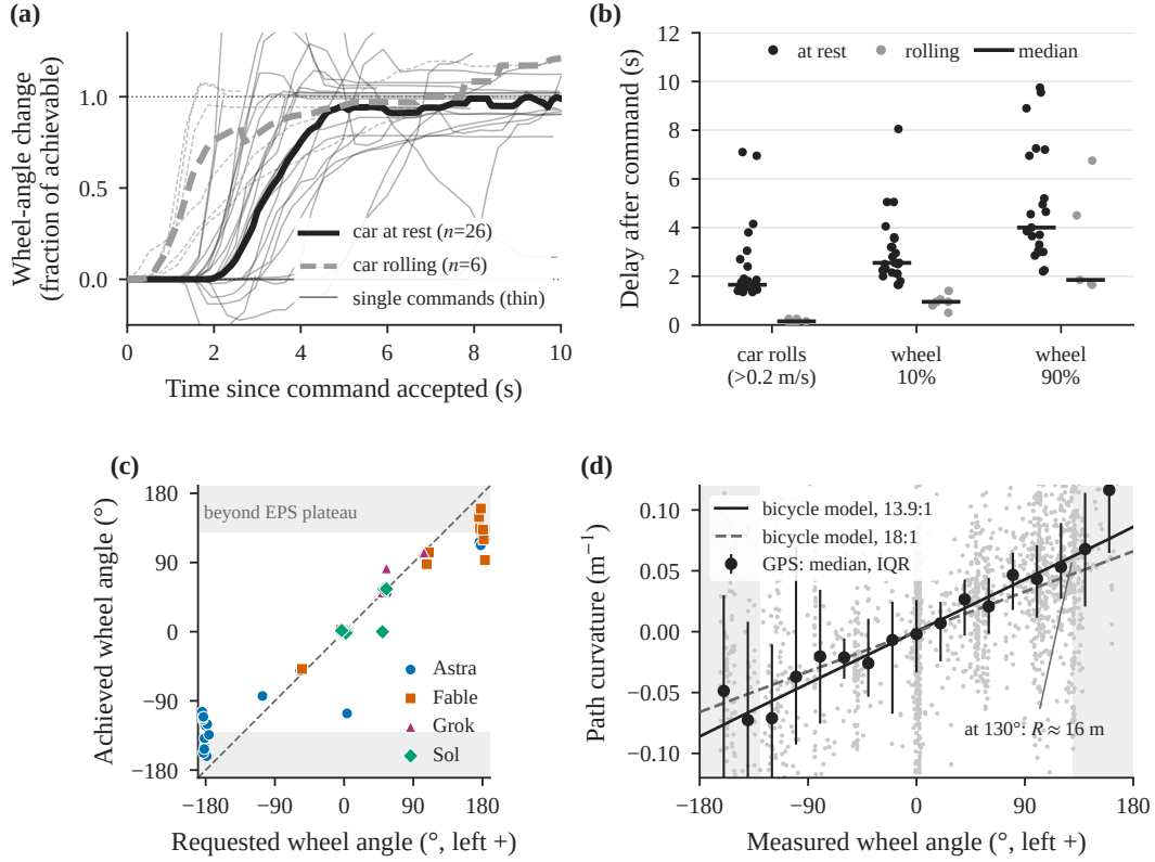
Figure 9: Requested versus actual steering. (a) Wheel-angle response to every command asking for a change of at least 30^\circ , normalized to the achievable change (request clipped to the \approx 130^\circ EPS plateau). Thick lines are medians. (b) Delays after a command is accepted. Of the 32 commands in (a), 26 arrived after the previous command had expired and the car had braked. The EPS only turns the wheel once the car rolls, so from rest the wheel reaches 90% of its change after a median of 4.0 s (1.9 s when already rolling). (c) Achieved versus requested wheel angle per command. Requests of 100% ( 180^\circ ) reach a median of 129^\circ , so the upper \approx 28\% of the command range wasn’t reached at the conditions of the model benchmark evaluations. (d) Measured path curvature from GPS against measured wheel angle, compared with a kinematic bicycle model. A 13.9:1 ratio fits better than the 18:1 in the harness documentation. At the plateau the turning radius is \approx 16 m, which implies roughly 25 s for a 90^\circ turn at 1 m/s, which is faster than the \sim 60 s we measured in a single sustained calibration run before the trial from rest and was used in the prompt’s example.
