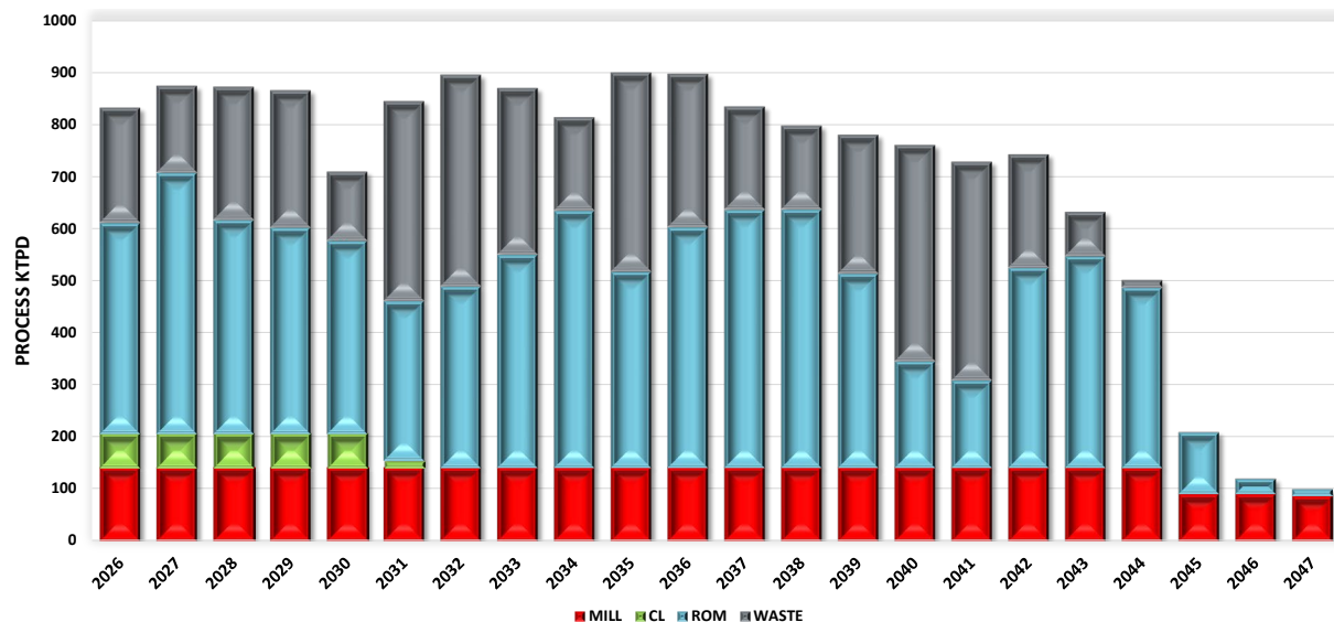
Figure 13.3 – Total Tonnage Planned Material Movement
