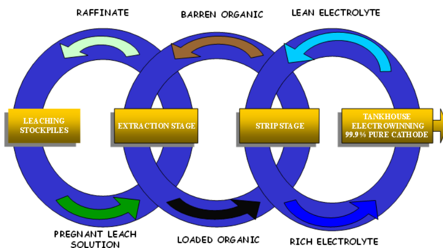
Figure 14.2 – Hydrometallurgical Transfer Process
