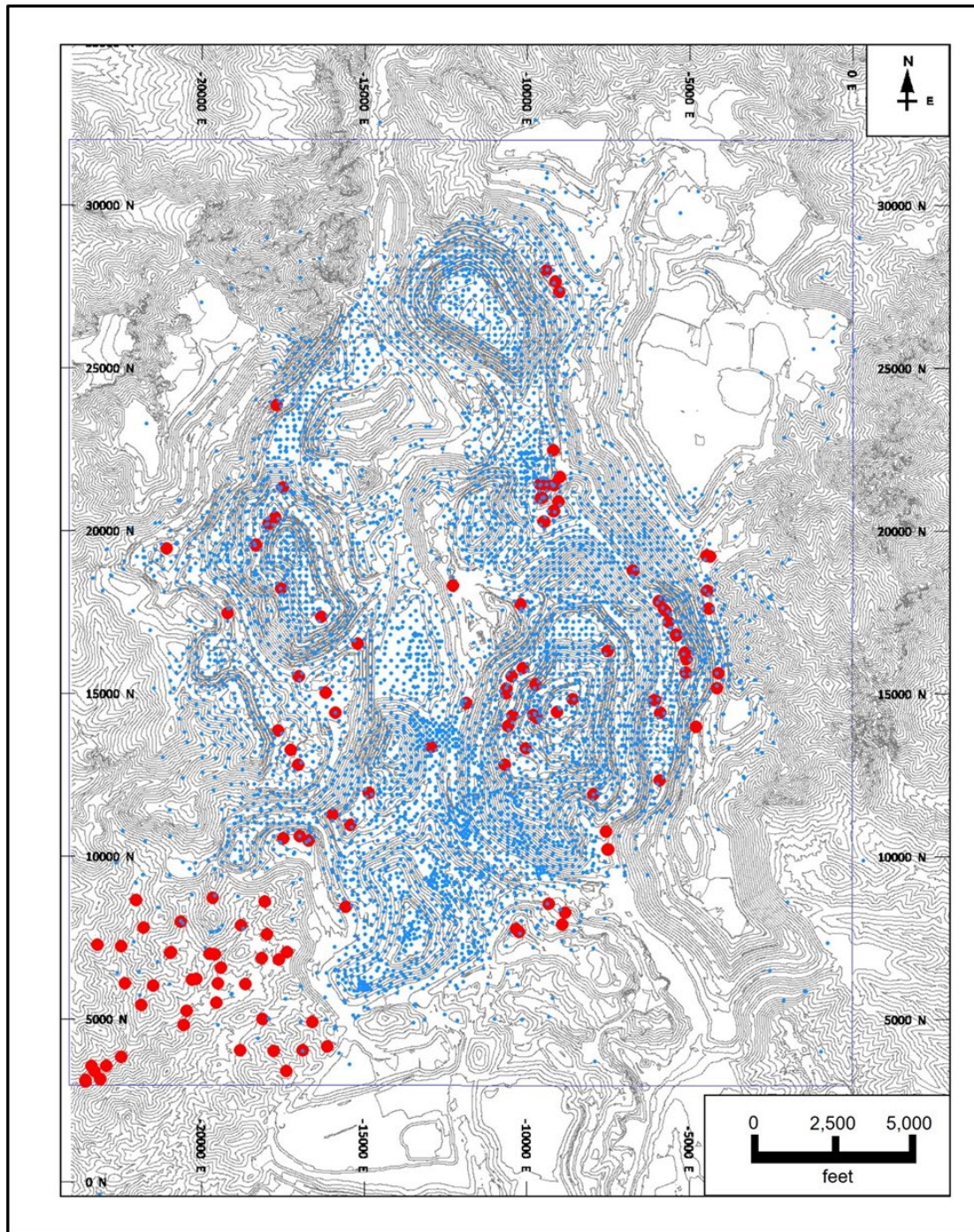
Figure 7.1 – Drill Hole Collar Locations
