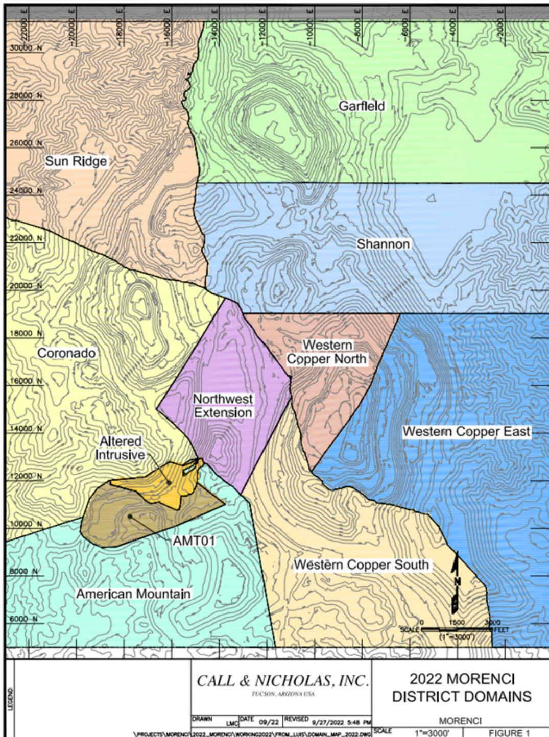
Figure 13.1 – Geotechnical Domains
