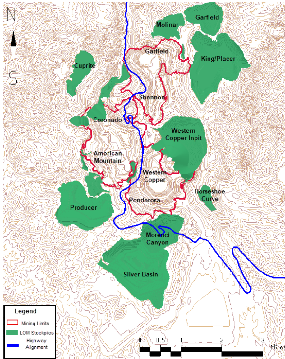
Figure 13.2 – Final Mine Design
