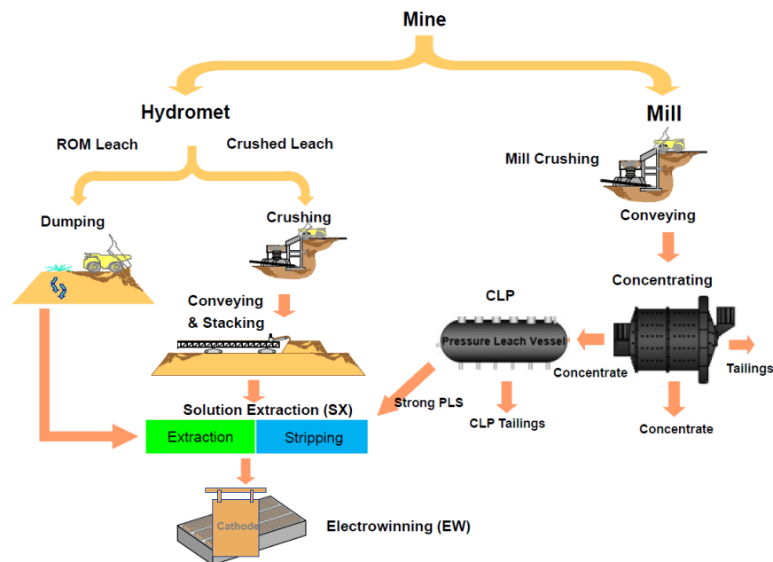
Figure 14.1 – Site Process Diagram
